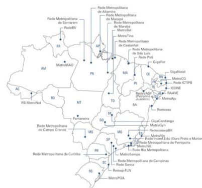
Fig. 11 Network maps of RNP – (a) national backbone, (b) location of the 40 metropolitan networks.
