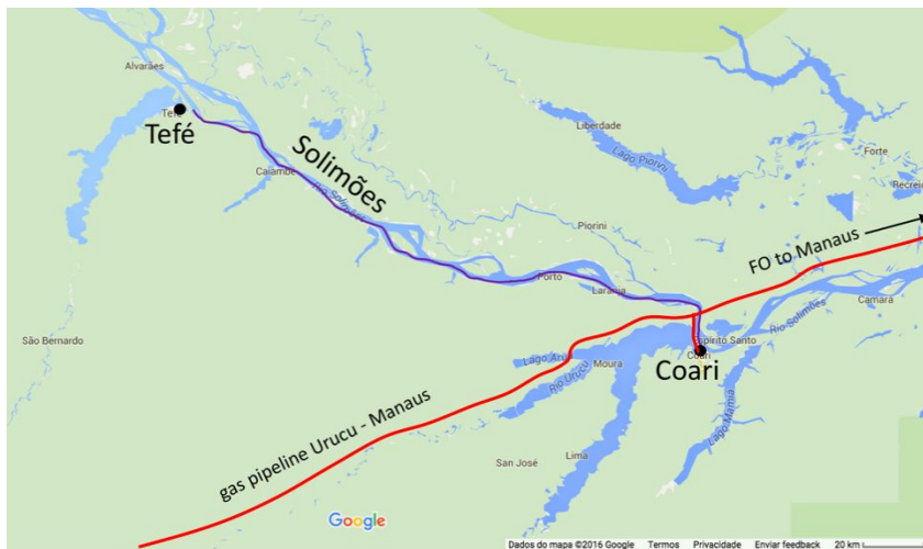
Fig. 18 The pilot project linking Coari to Tefé along the Solimões.
