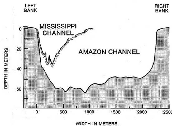
Fig. 7 A comparison of the shape of the Mississippi and the Amazon at their deepest points, Vicksburg, MS, (1 km wide and 38 m deep) and Obidos, PA (2 km wide and 60 m deep). 7
